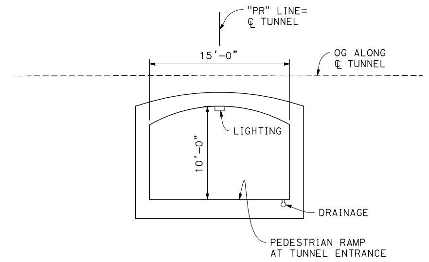
SECTION A-A 1" = 5'
