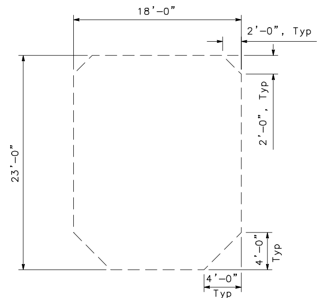
PERMANENT CLEARANCE ZONE NO SCALE
