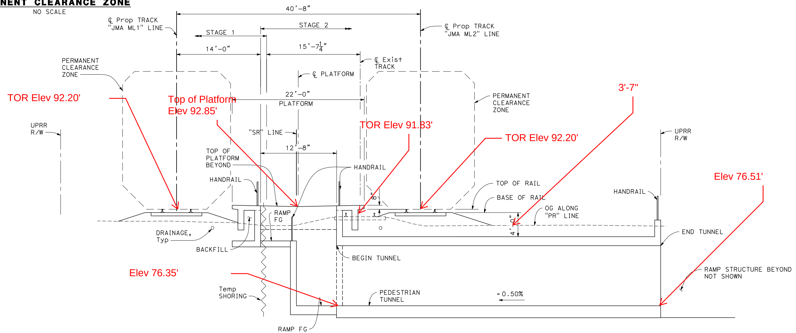
SECTION B-B 1" = 5'
