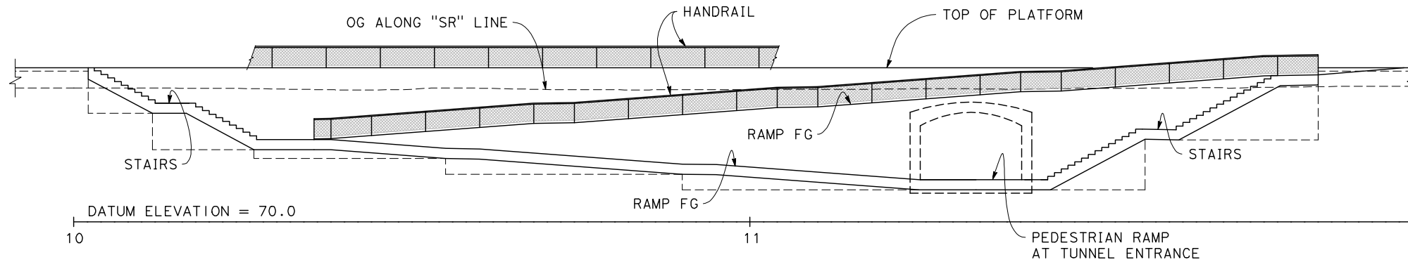
ELEVATION ALONG "SR" LINE 1" = 20'
